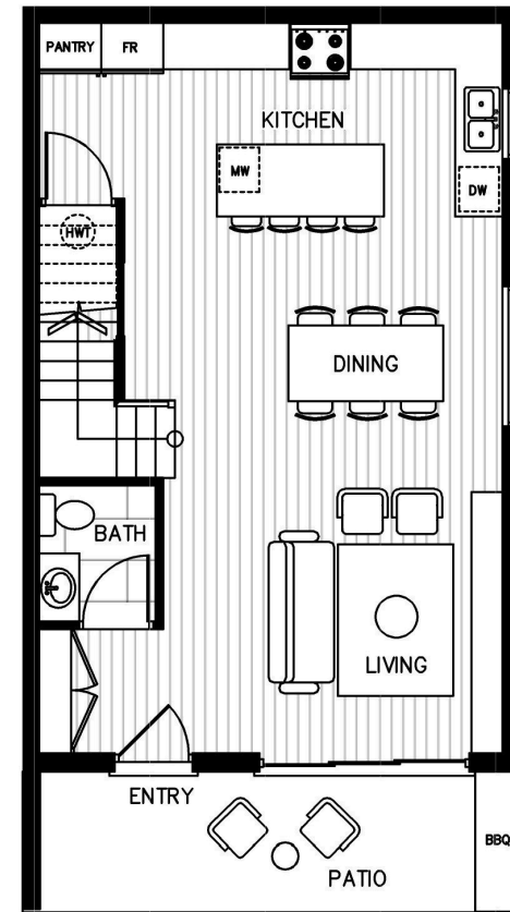
LEVEL ONE 664 SQ FT
